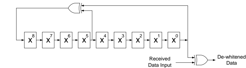
Figure 45. Whitening/De-Whitening Algorithm Structure
