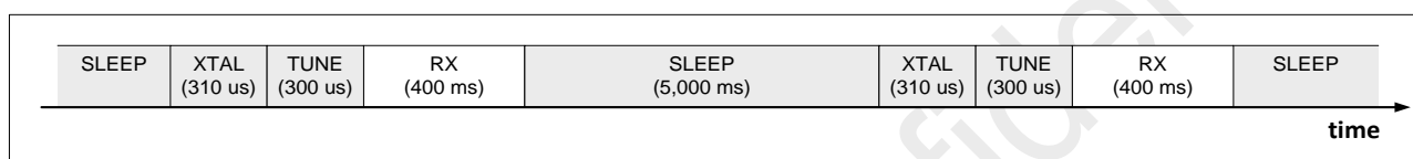
Figure 21. Fixed Duty Operation
